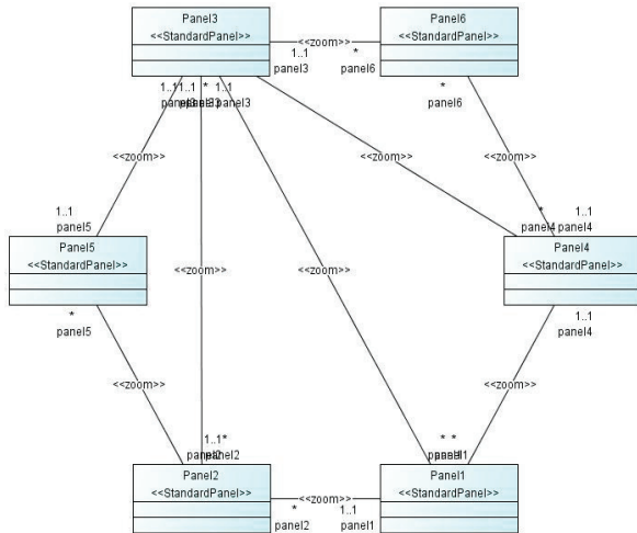
Figure 5.2 An example of a class diagram arranged using the circular graph drawing algorithm
